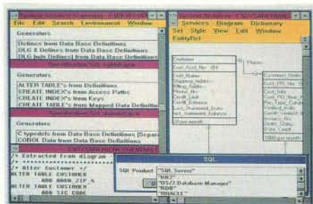
Generate schema from entity diagrams.
